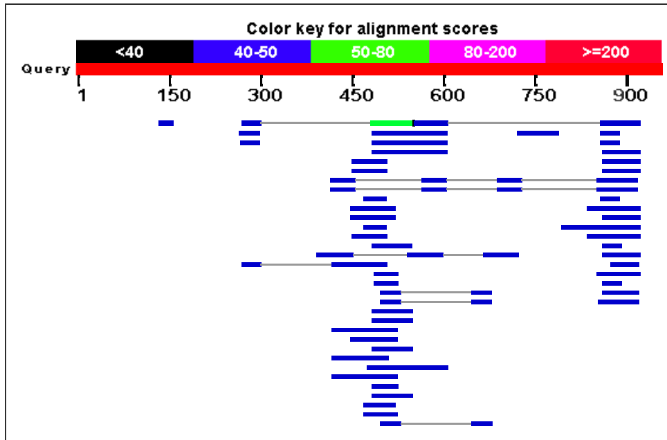
Distribution of 83 Blast Hits on the Query Sequence
